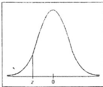
(a) Table of Areas to the Left of z
