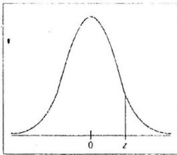
Areas of a Standard Normal Distribution continued
